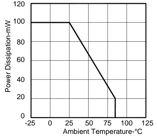
FIG.2 Power Dissipation Vs. Ambient Temperature (mW)
