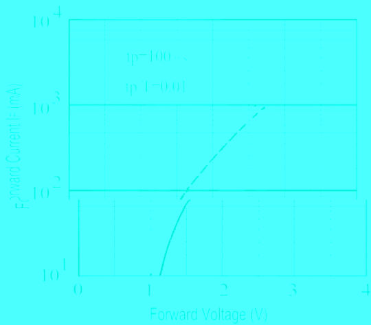
Forward Voltage
